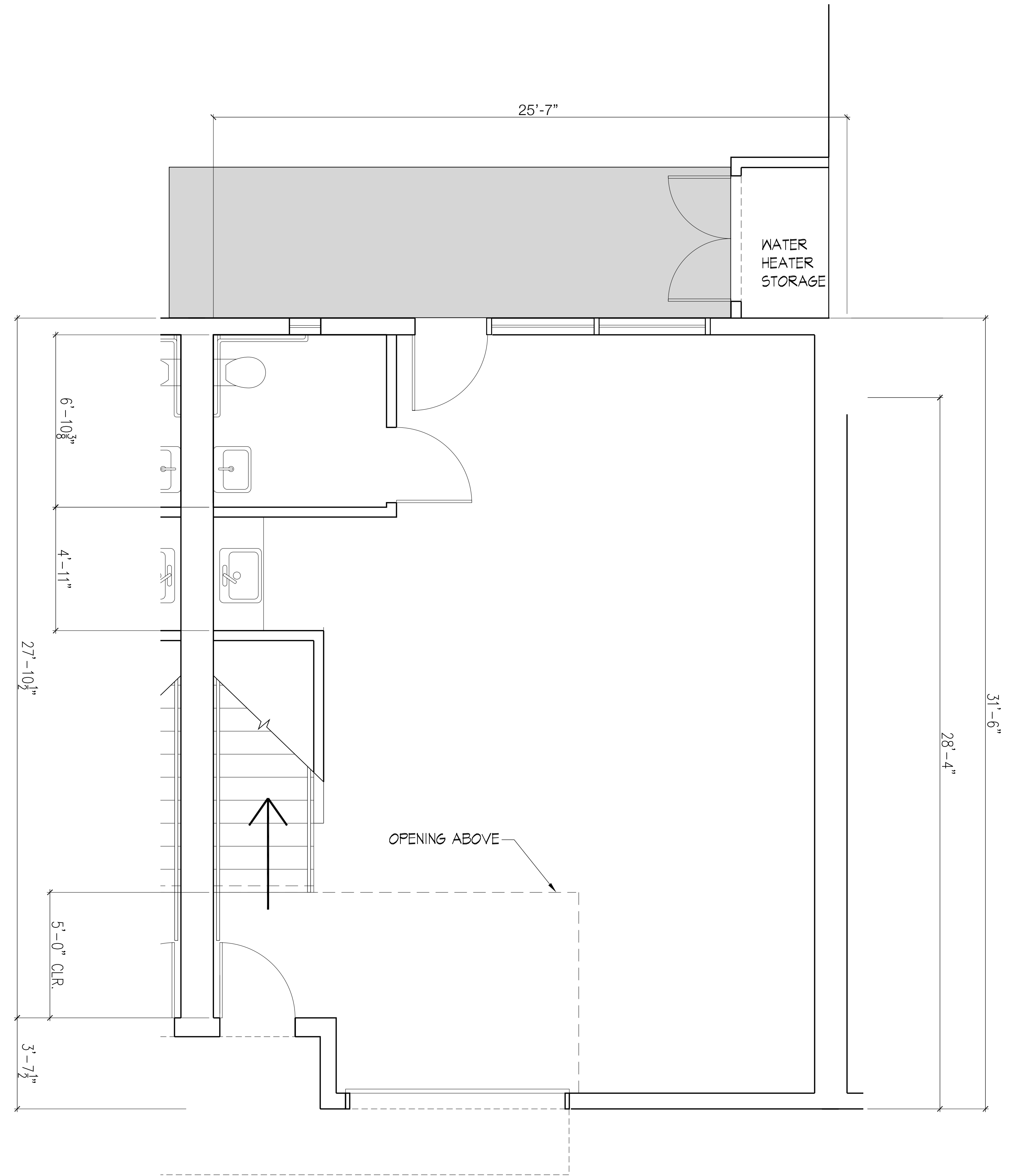
1 Unit F 1st Floor Plan 3/8" = 1'-0"
