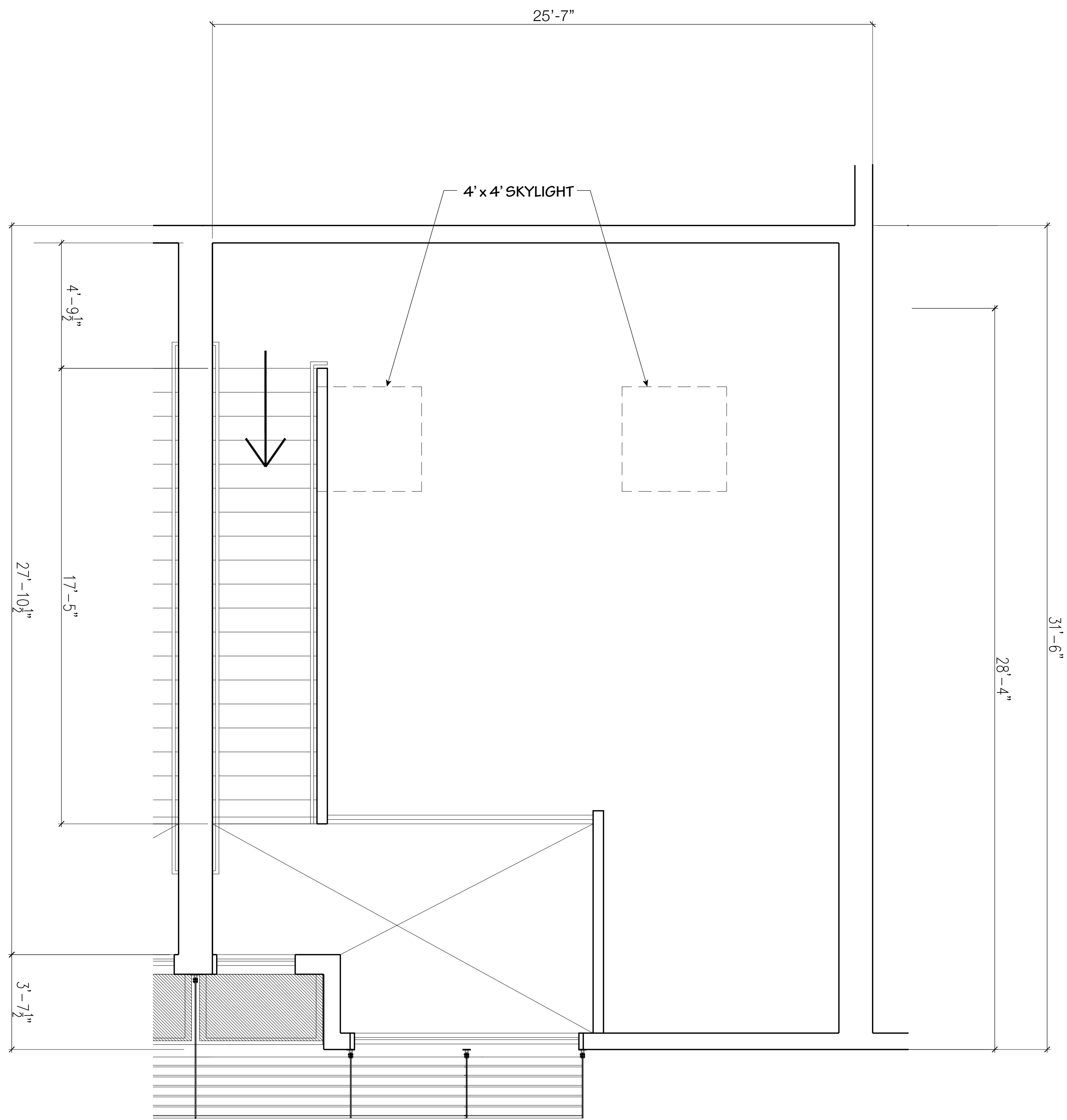
2 Unit F 2nd Floor Plan 3/8" = 1'-0"
